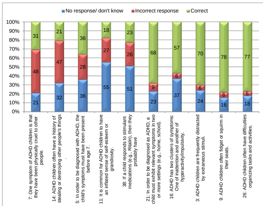
Figure 2. Categorised responses to Symptoms/ Diagnosis items
